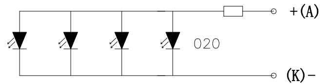
BACKLIGHT CIRCUIT BLUE if=60mA & Vf=3.0V TYPE
